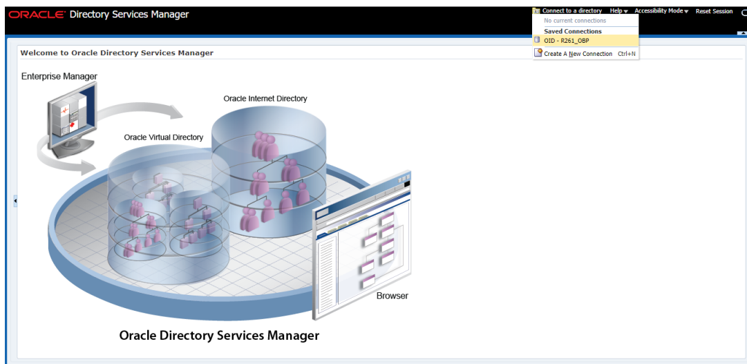
Figure 6–1 Opening ODSM
